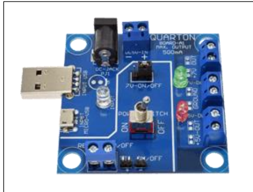
Multi-function Laser Module Power Supply Board.
