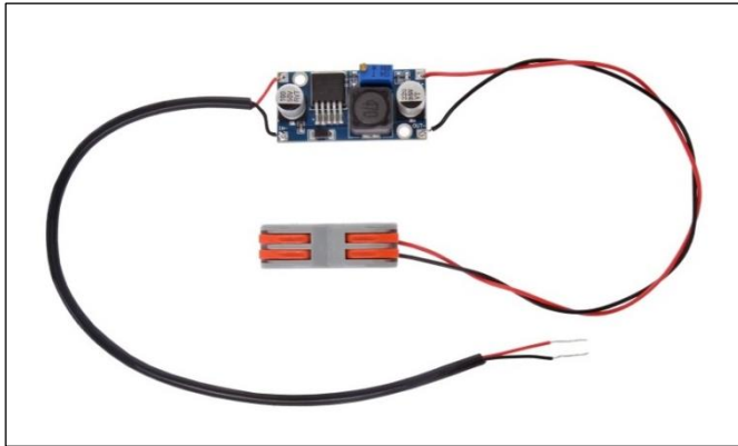
DC converter : In 9~36V, Out 5V 1A.
